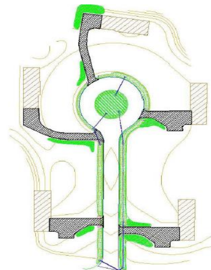
Figure 3.7 – Cul-de-sac designs.
